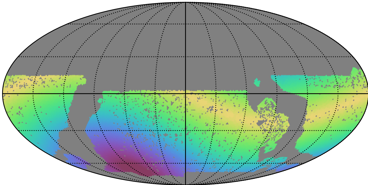
baseline_v3.0_10yrs WFD y band: Max solarElong
