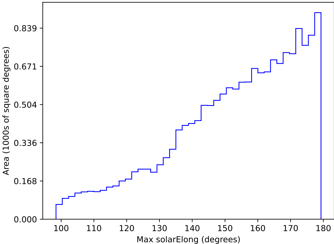
baseline_v3.0_10yrs WFD y band: Max solarElong
