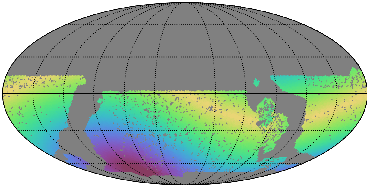
baseline_v3.0_10yrs WFD u band: Max solarElong
