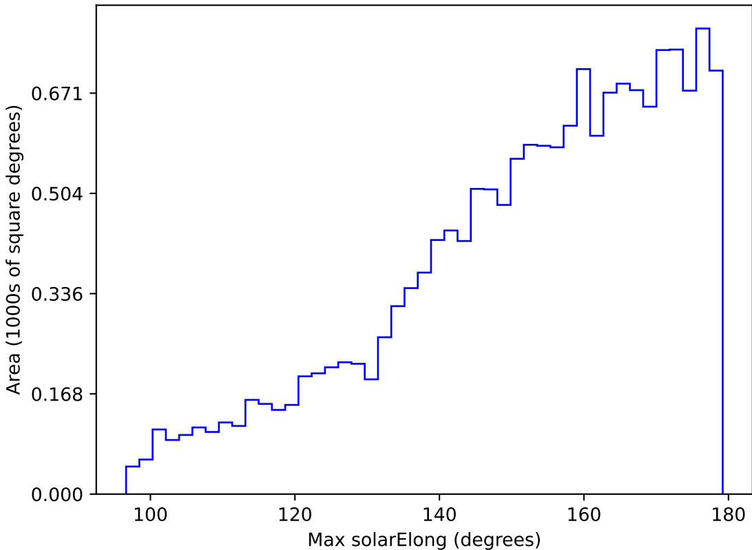
baseline_v3.0_10yrs WFD u band: Max solarElong
