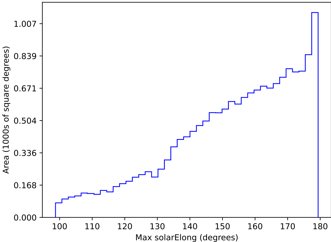
baseline_v3.0_10yrs WFD r band: Max solarElong
