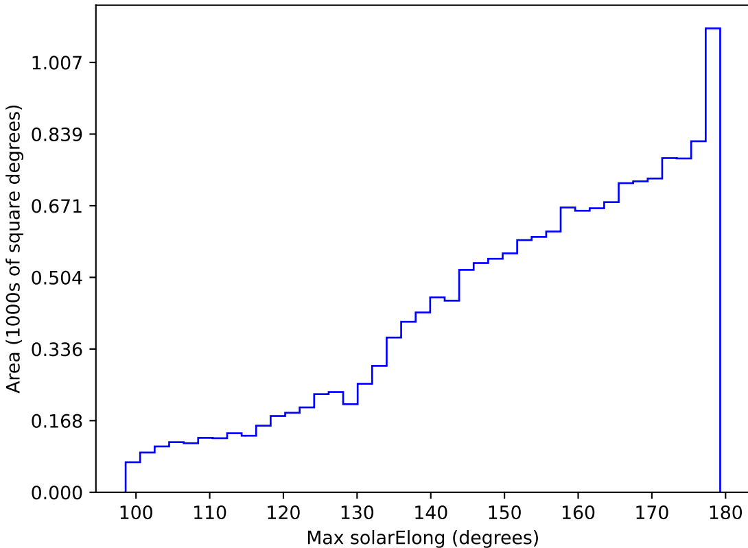
baseline_v3.0_10yrs WFD i band: Max solarElong
