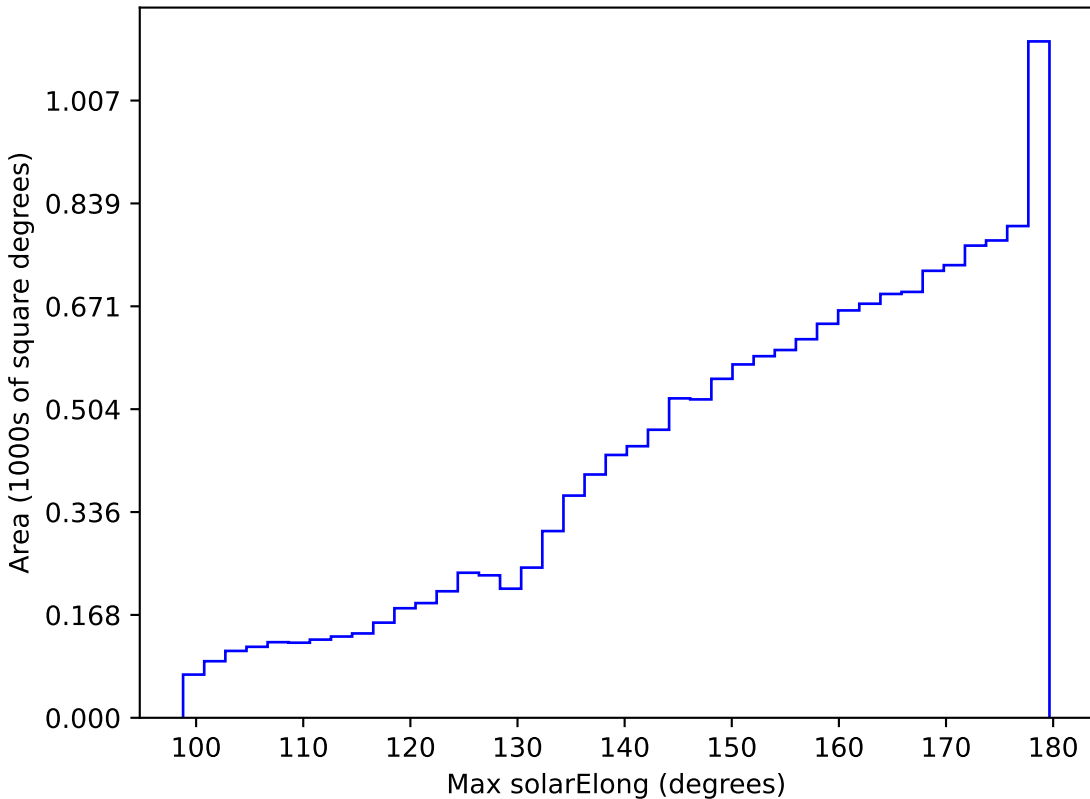
baseline_v3.0_10yrs WFD all bands: Max solarElong
