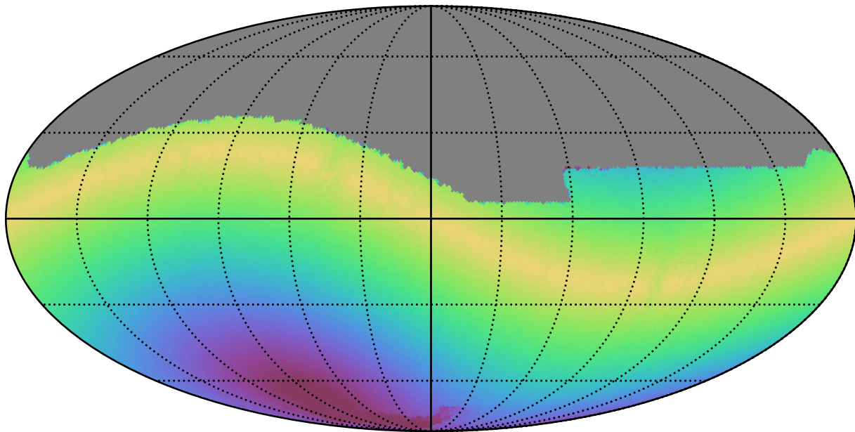
baseline_v3.0_10yrs All sky z band: Max solarElong
