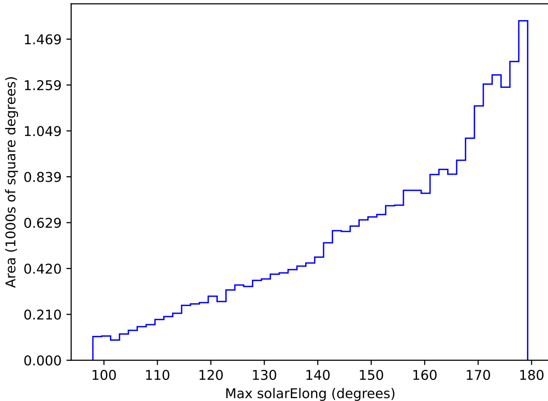
baseline_v3.0_10yrs All sky z band: Max solarElong
