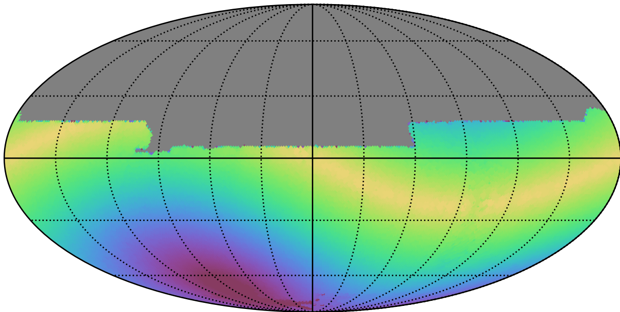
baseline_v3.0_10yrs All sky y band: Max solarElong
