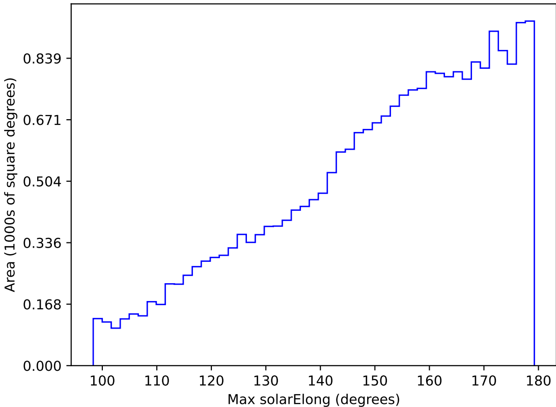
baseline_v3.0_10yrs All sky y band: Max solarElong
