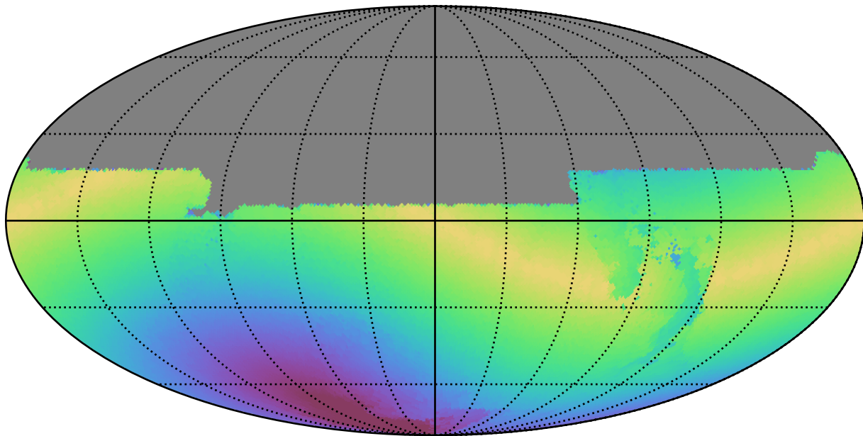
baseline_v3.0_10yrs All sky u band: Max solarElong
