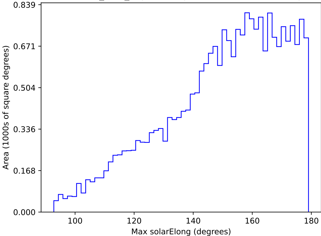
baseline_v3.0_10yrs All sky u band: Max solarElong
