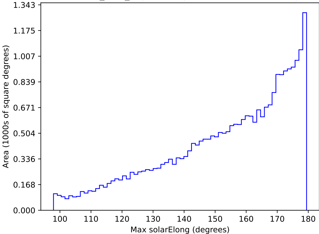
baseline_v3.0_10yrs All sky r band: Max solarElong
