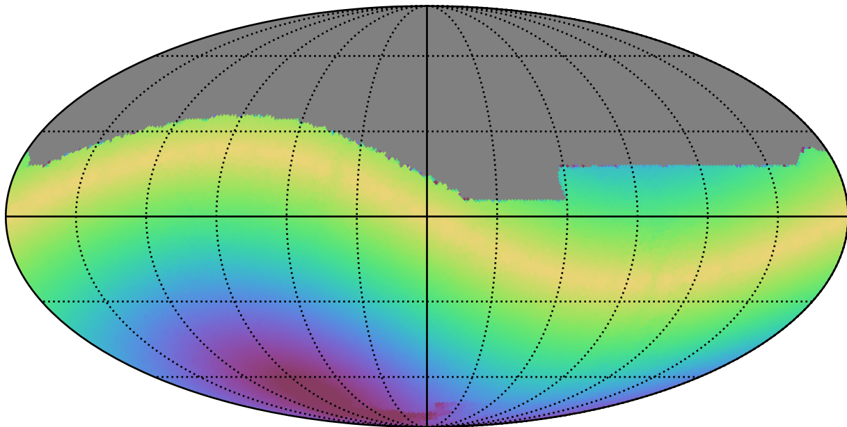
baseline_v3.0_10yrs All sky i band: Max solarElong
