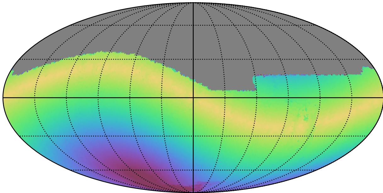
baseline_v3.0_10yrs All sky g band: Max solarElong
