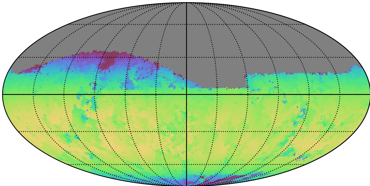
baseline_v3.0_10yrs Yr 1 z band: Max skyBrightness
