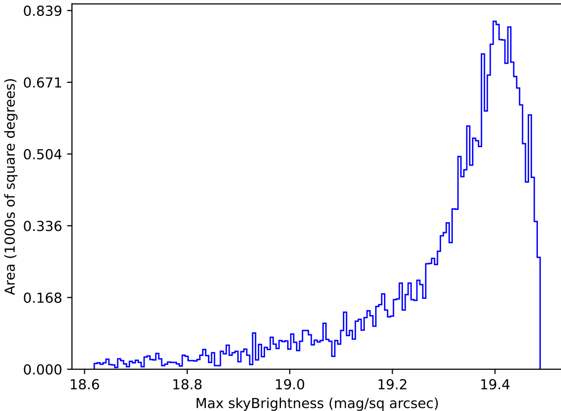
baseline_v3.0_10yrs Yr 1 z band: Max skyBrightness
