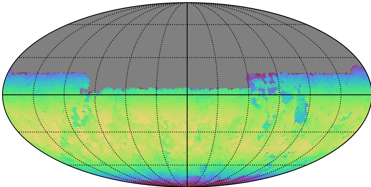
baseline_v3.0_10yrs Yr 1 y band: Max skyBrightness
