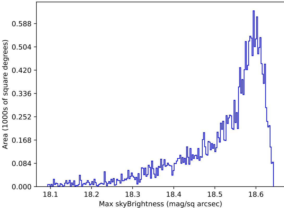
baseline_v3.0_10yrs Yr 1 y band: Max skyBrightness
