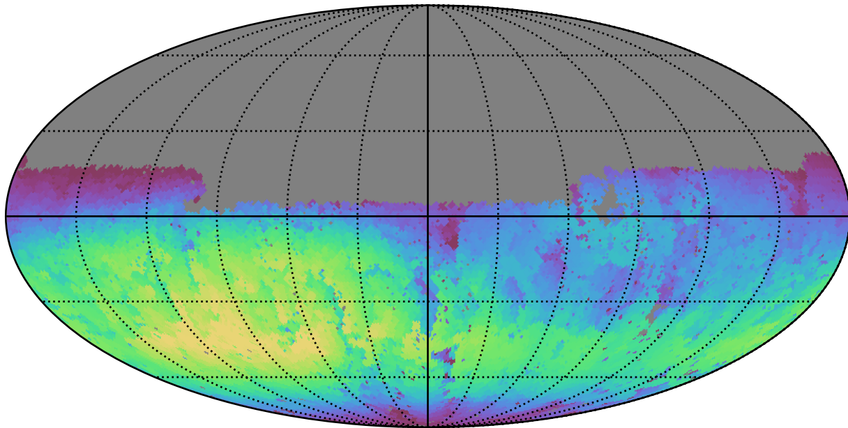
baseline_v3.0_10yrs Yr 1 u band: Max skyBrightness
