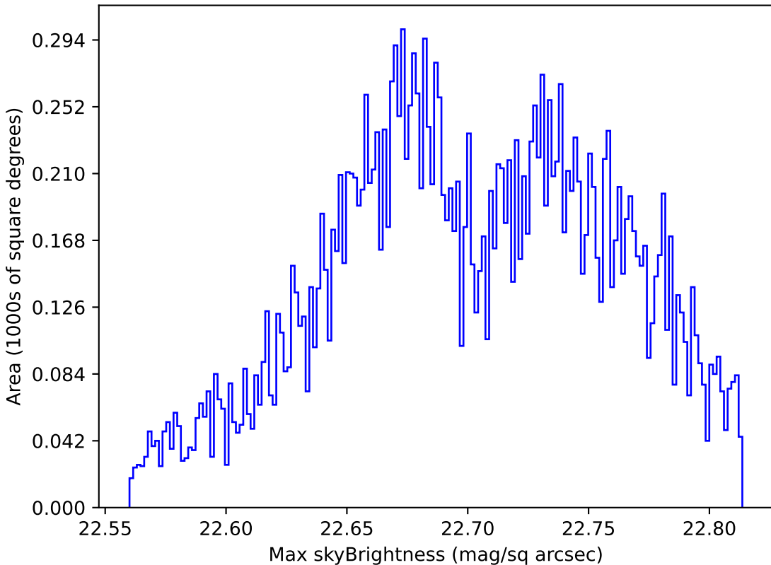
baseline_v3.0_10yrs Yr 1 u band: Max skyBrightness
