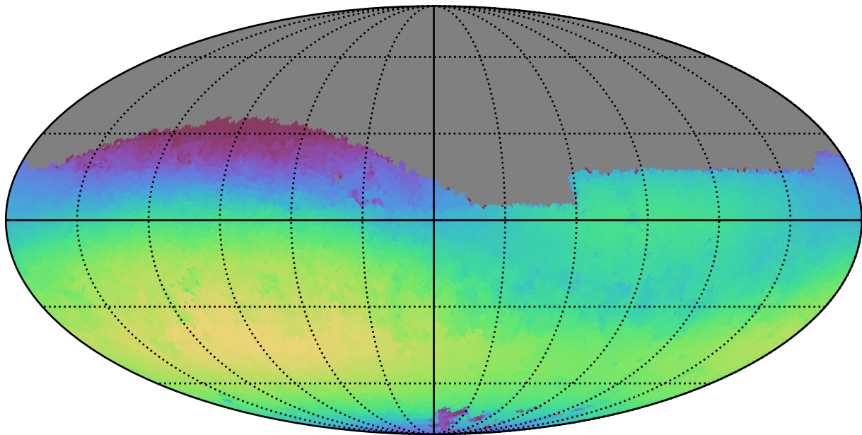
baseline_v3.0_10yrs Yr 1 r band: Max skyBrightness
