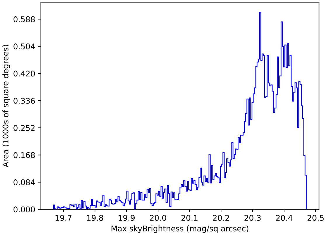
baseline_v3.0_10yrs Yr 1 i band: Max skyBrightness
