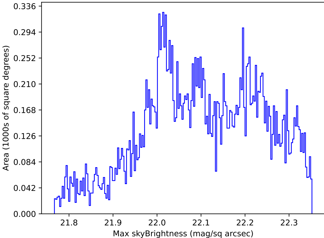
baseline_v3.0_10yrs Yr 1 g band: Max skyBrightness
