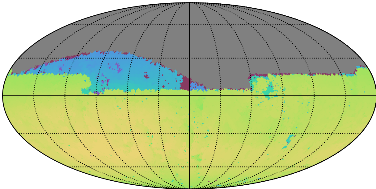
baseline_v3.0_10yrs Yr 1 all bands: Max skyBrightness
