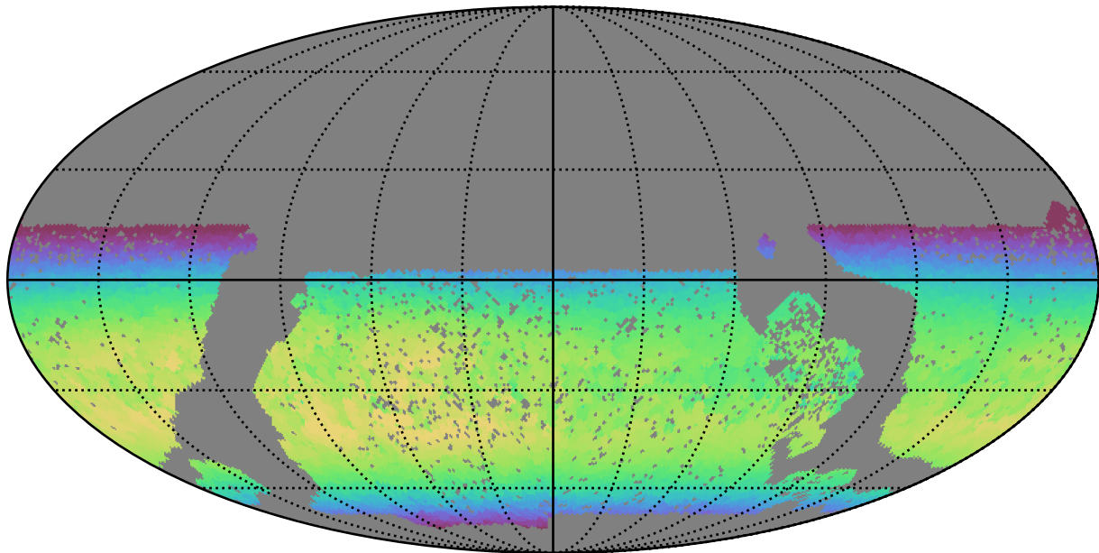
baseline_v3.0_10yrs WFD z band: Max skyBrightness
