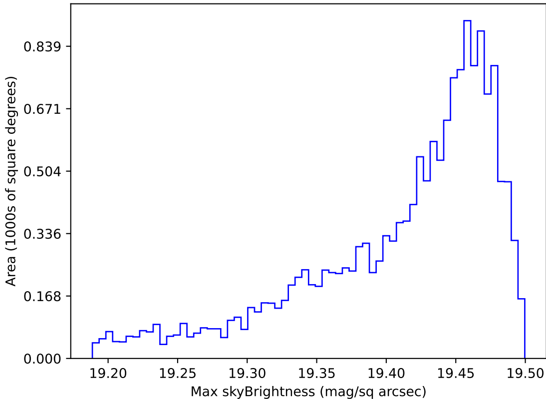
baseline_v3.0_10yrs WFD z band: Max skyBrightness
