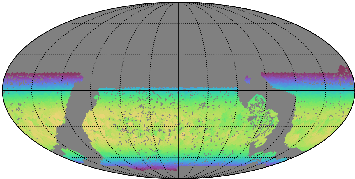
baseline_v3.0_10yrs WFD y band: Max skyBrightness
