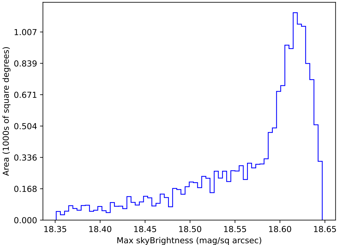
baseline_v3.0_10yrs WFD y band: Max skyBrightness
