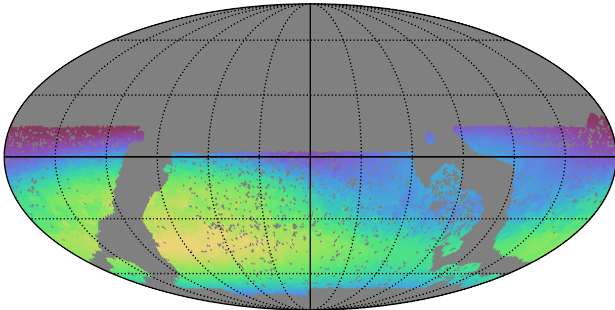
baseline_v3.0_10yrs WFD u band: Max skyBrightness
