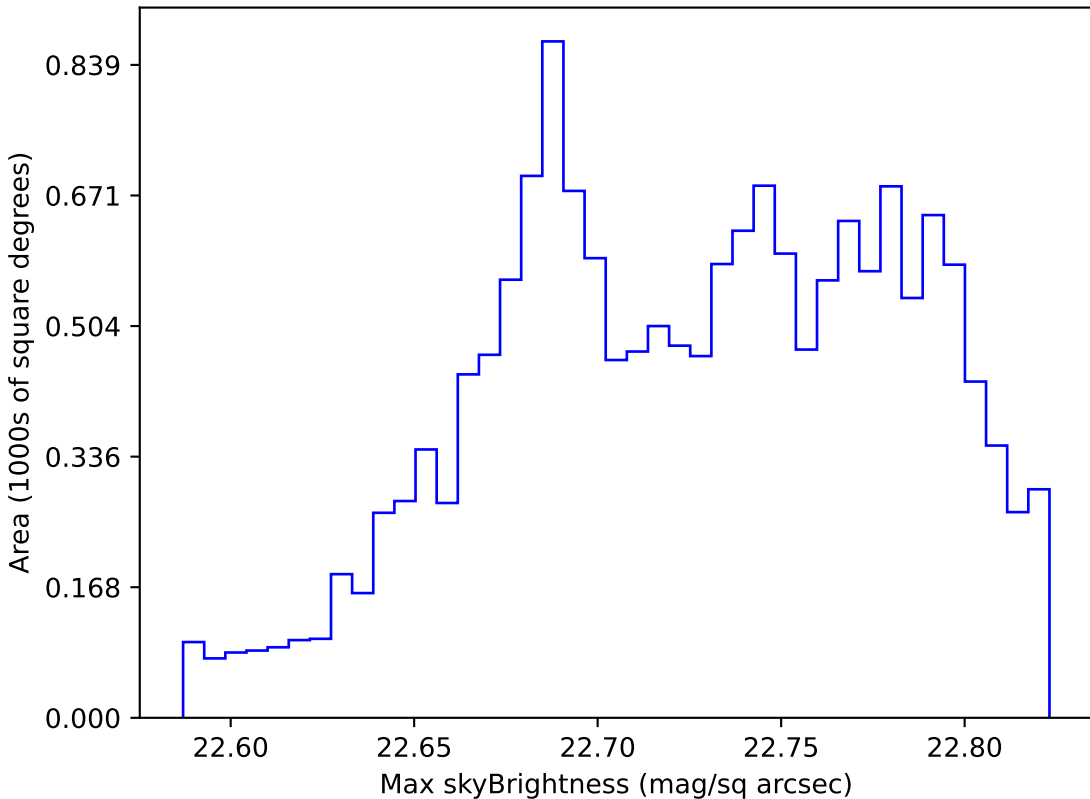
baseline_v3.0_10yrs WFD u band: Max skyBrightness
