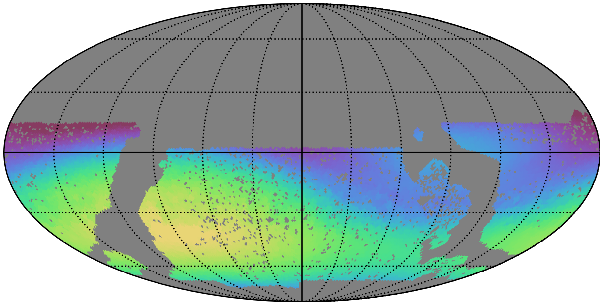
baseline_v3.0_10yrs WFD r band: Max skyBrightness
