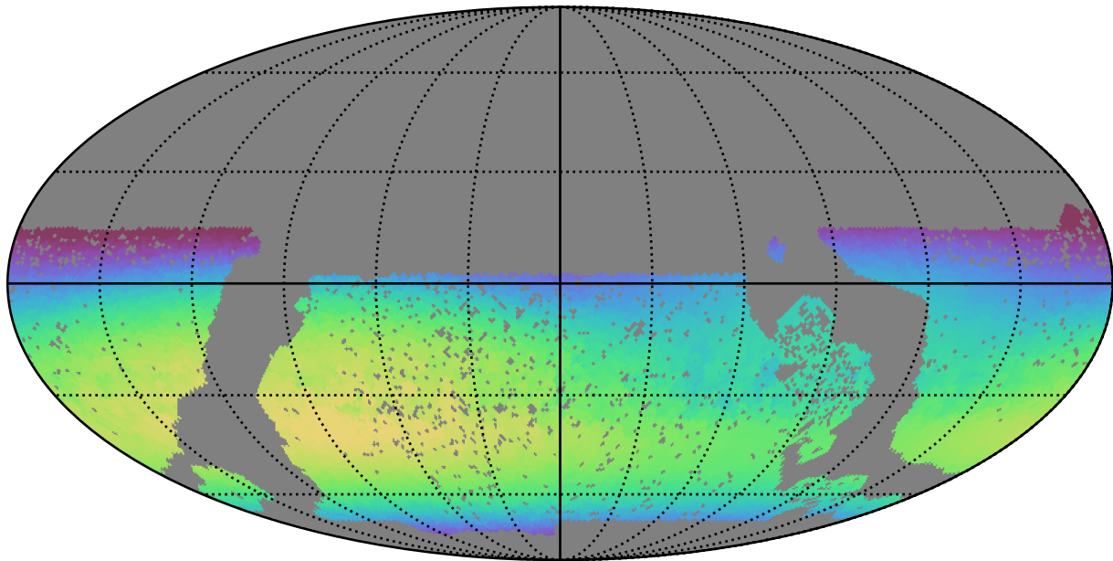
baseline_v3.0_10yrs WFD i band: Max skyBrightness
