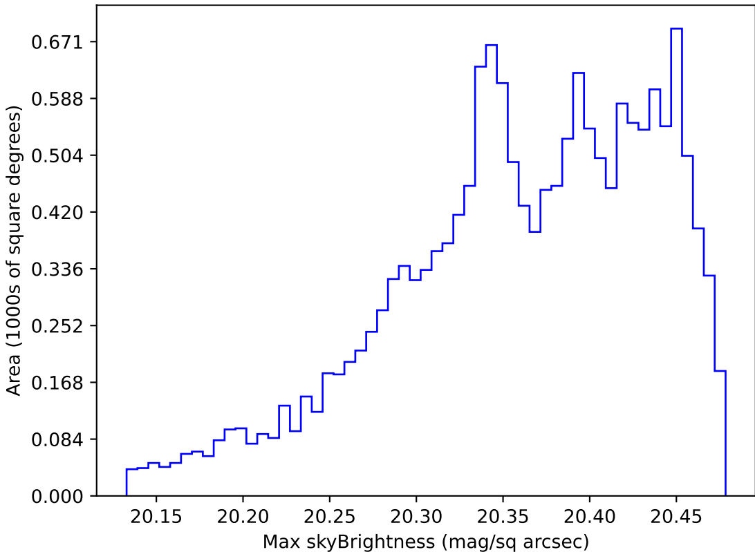
baseline_v3.0_10yrs WFD i band: Max skyBrightness
