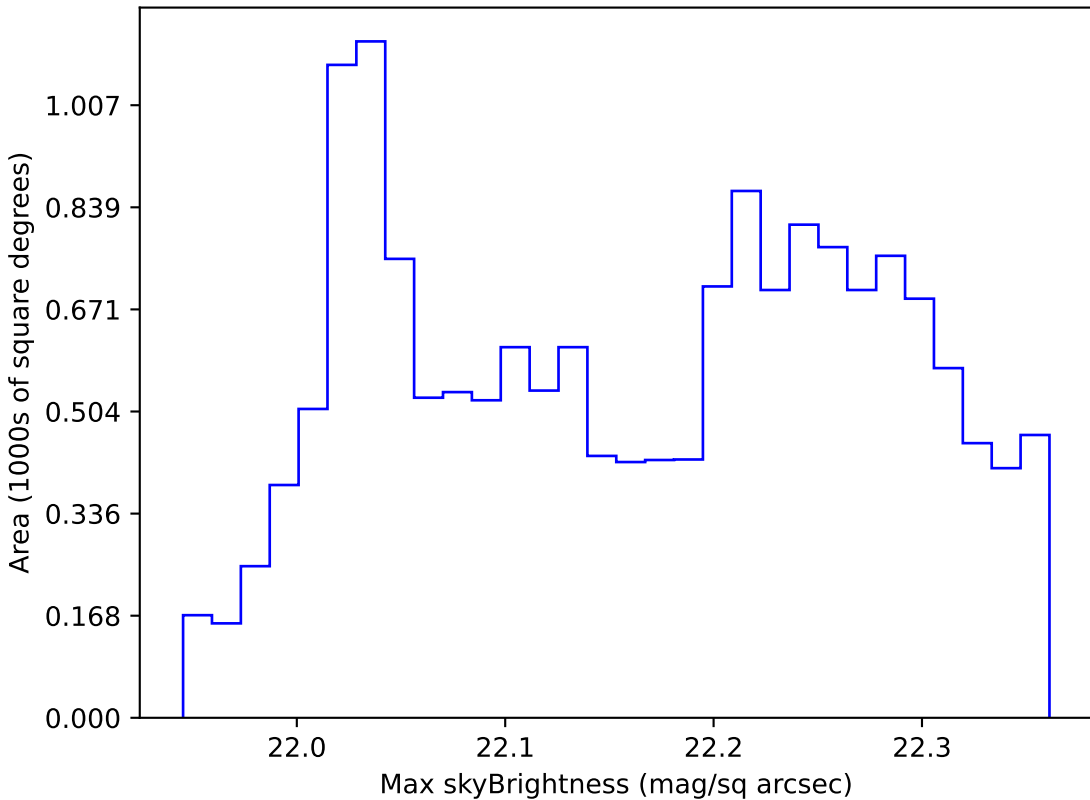
baseline_v3.0_10yrs WFD g band: Max skyBrightness
