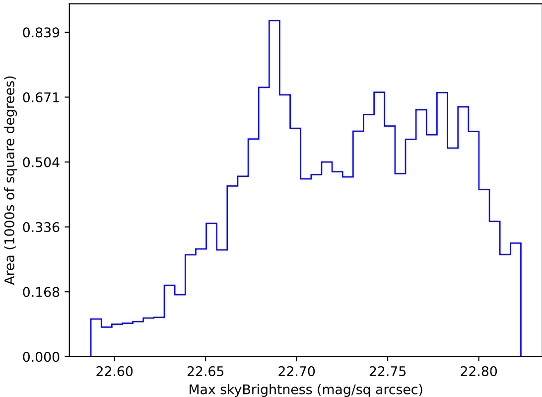
baseline_v3.0_10yrs WFD all bands: Max skyBrightness
