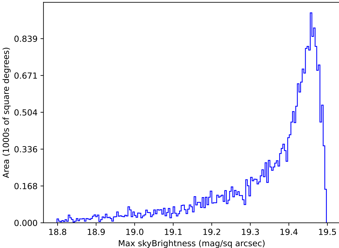
baseline_v3.0_10yrs All sky z band: Max skyBrightness
