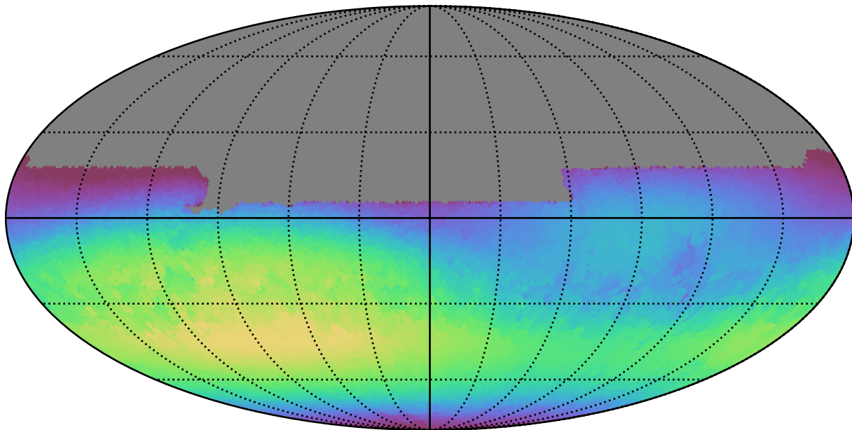
baseline_v3.0_10yrs All sky u band: Max skyBrightness
