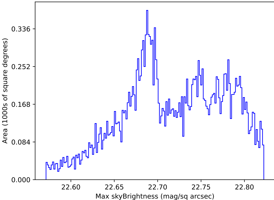
baseline_v3.0_10yrs All sky u band: Max skyBrightness
