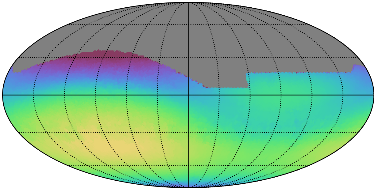
baseline_v3.0_10yrs All sky r band: Max skyBrightness
