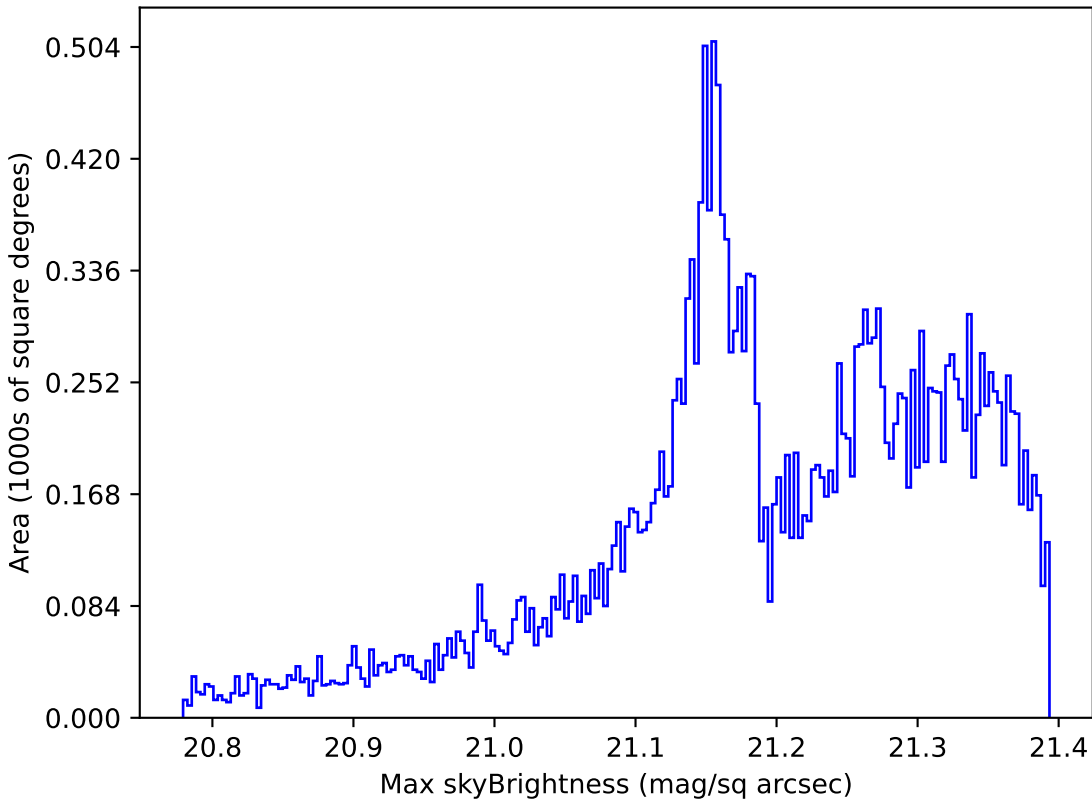
baseline_v3.0_10yrs All sky r band: Max skyBrightness
