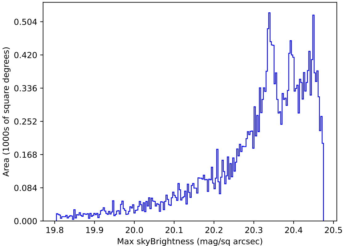
baseline_v3.0_10yrs All sky i band: Max skyBrightness
