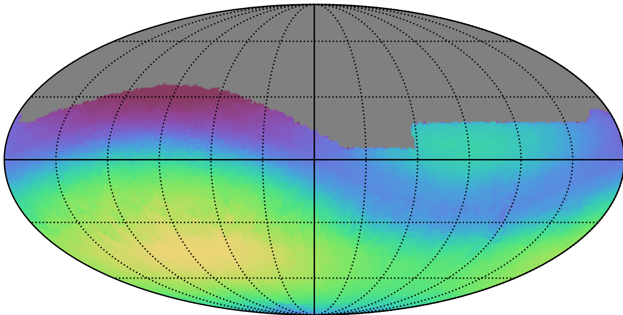
baseline_v3.0_10yrs All sky g band: Max skyBrightness
