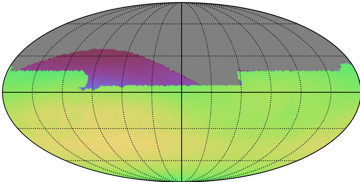
baseline_v3.0_10yrs All sky all bands: Max skyBrightness
