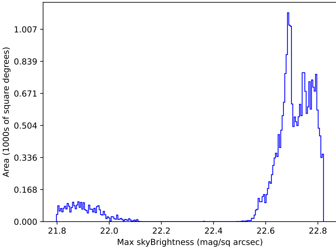
baseline_v3.0_10yrs All sky all bands: Max skyBrightness
