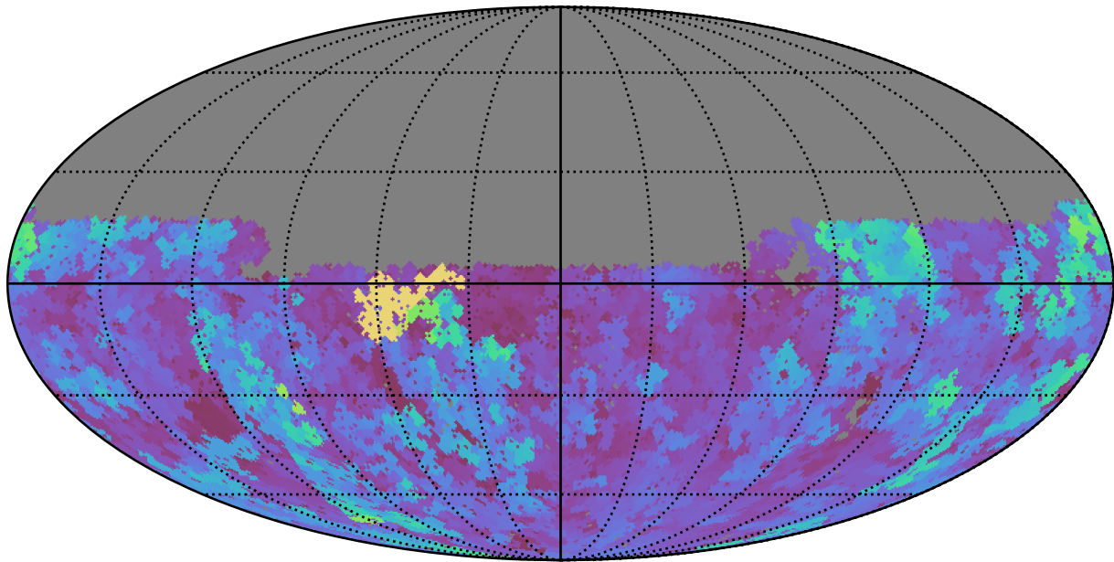
baseline_v3.0_10yrs Yr 1 u band: Max seeingGeom
