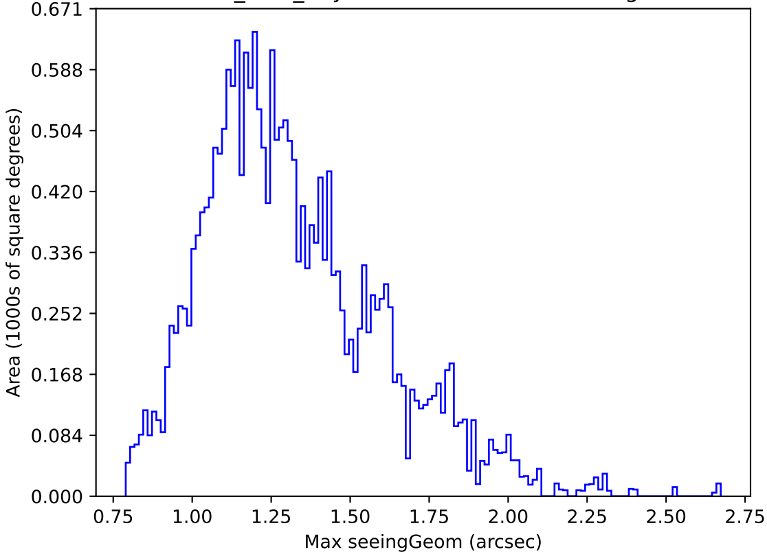
baseline_v3.0_10yrs Yr 1 u band: Max seeingGeom
