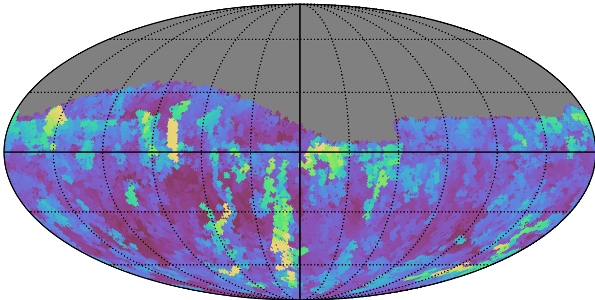
baseline_v3.0_10yrs Yr 1 r band: Max seeingGeom
