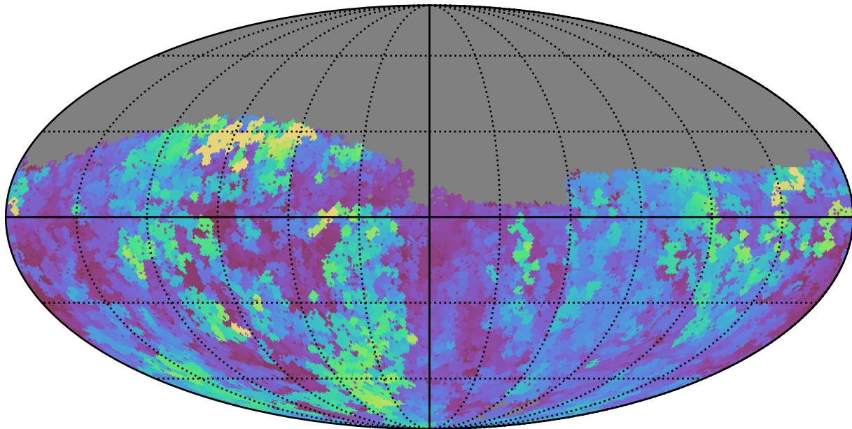
baseline_v3.0_10yrs Yr 1 g band: Max seeingGeom
